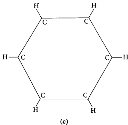
9.21 Three carbon-hydrogen bond structures: (a) Ethylene C_2H_4 ; (b) Acetylene C_2H_2 ; (c) Benzene C_6H_6 .
